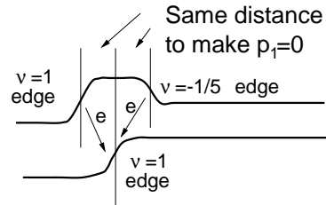
FIG. 2. The edge of \nu = 9/5 bilayer state and the charge transfer caused by the V_{\mathbf{m}_1} operator.
