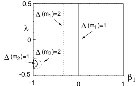
FIG. 1. Plot of scaling dimension of the two neutral null operators for \nu = 9/5 edge as functions of (\beta_1, \lambda) . Dash lines indicate when operators become marginal ( \Delta(\mathbf{m}) = 2 ) and solid lines indicate the soluble case where ( \Delta(\mathbf{m}) = 1 ).
