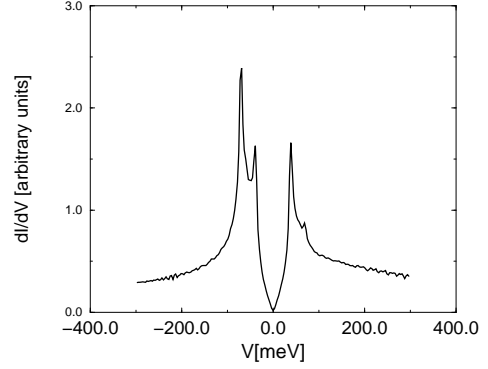
FIG. 1. The two peaks symmetrically located in height and energy with respect to zero bias are the usual peaks arising from the gap structure in the superconducting density of states. The two outer peaks are the remnants of the van Hove singularity. The wiggles in the background are due to the discreteness of k-space when performing numerical calculation. The discreteness gets amplified by the derivative taken in obtaining \frac{dI}{dV} from the tunneling current (3). The resolution in voltage is 3meV
