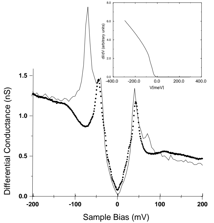
FIG. 2. Here we have set t_1^f/2t^b = 1/2 . \Delta^f = \Delta_0^f(\cos k_x - \cos k_y) and \Delta^b = \Delta_0^b(\cos k_x - \cos k_y) with \Delta_0^f/\Delta_0^b = 1/2 where t_1^f = -297.6 meV from the ARPES fit and \Delta_0^f = 22 meV. Notice that above ratios correspond to J/t = 1/2 within the t-J model. The solid curve is our slave-boson result. The wiggles in the background are more pronounced here as compared with Fig. (1) due to smaller resolution in k-space in calculating the convolution integrals (4). Here the resolution in V is 5 meV. The dots are the experimental result from Ref. [2]. The inset shows the incoherent part of the hole tunneling spectral weight. Notice that the exact shape of this curve should not be taken too literally - see discussion on boson band structure in the main text.
