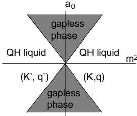
FIG. 1. The phase diagram near a critical point.
